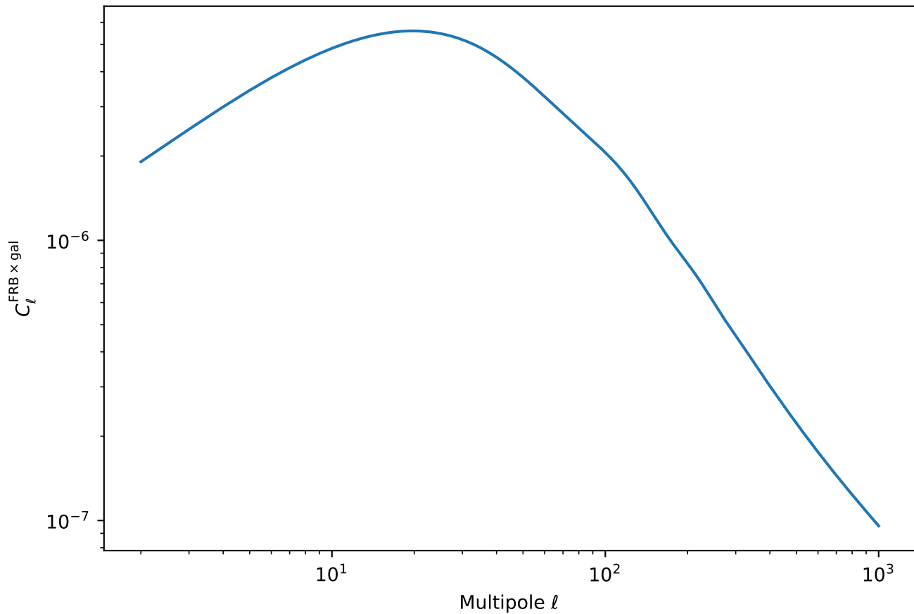
FRB×Galaxy Cross-Correlation (Neutron Stars, Shallow Survey, Galaxy Bin 3)
