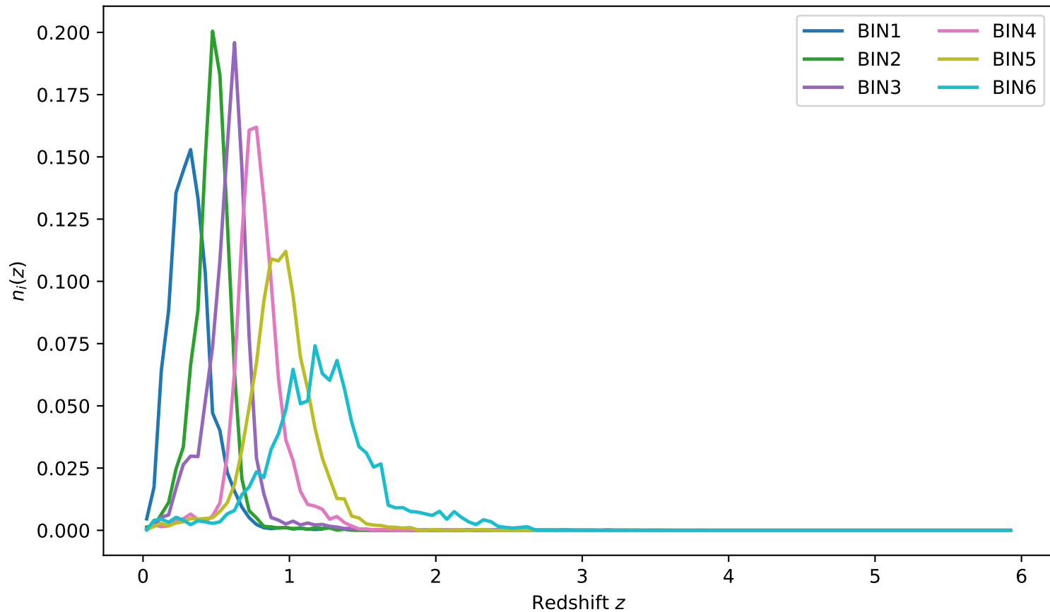
Galaxy Tomographic Redshift Distributions
