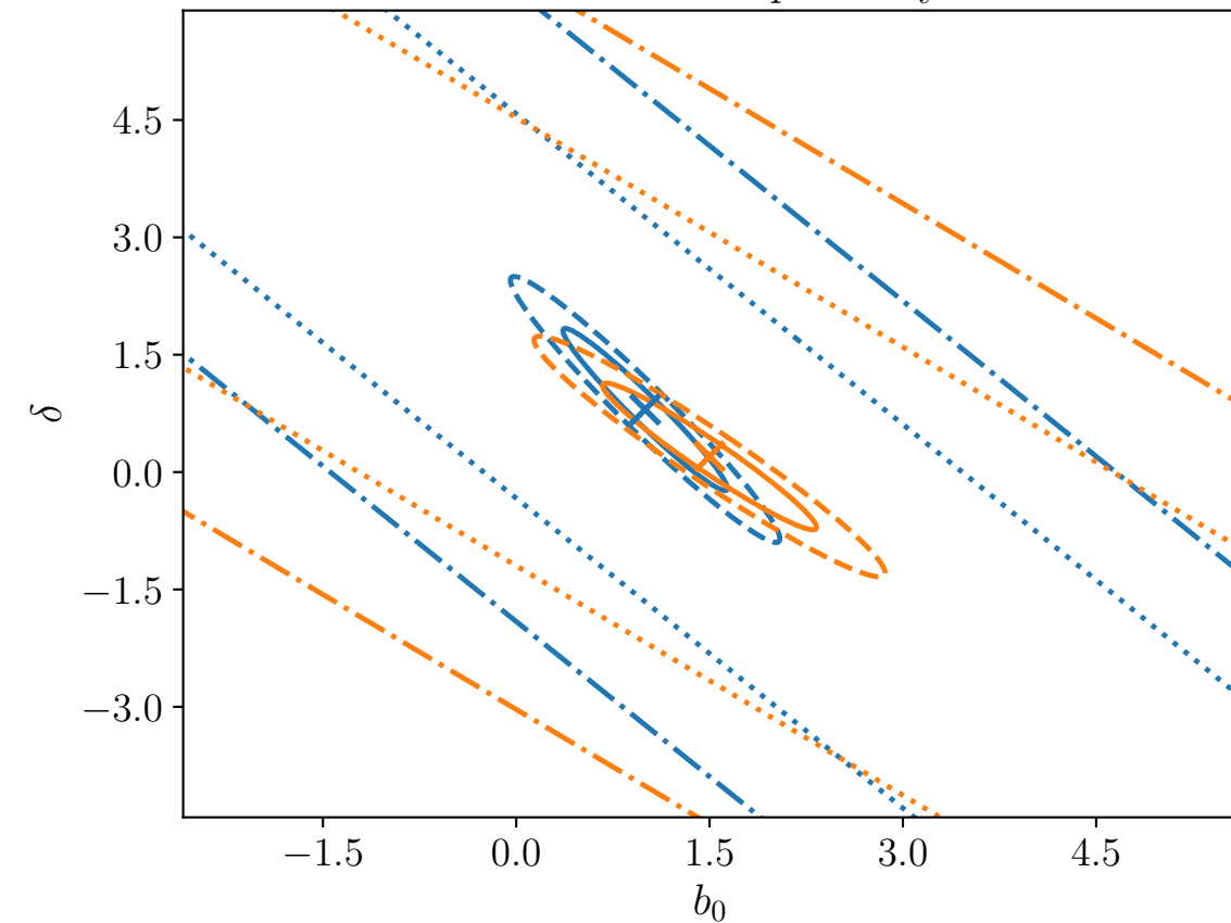
LSST Y10 Deep Survey
