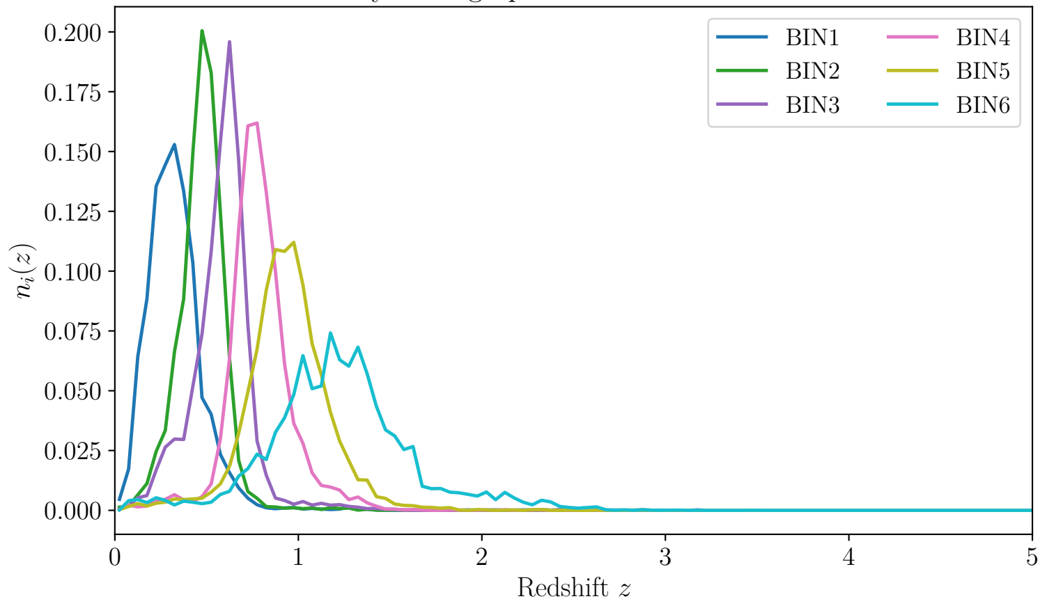
Galaxy Tomographic Redshift Distributions
