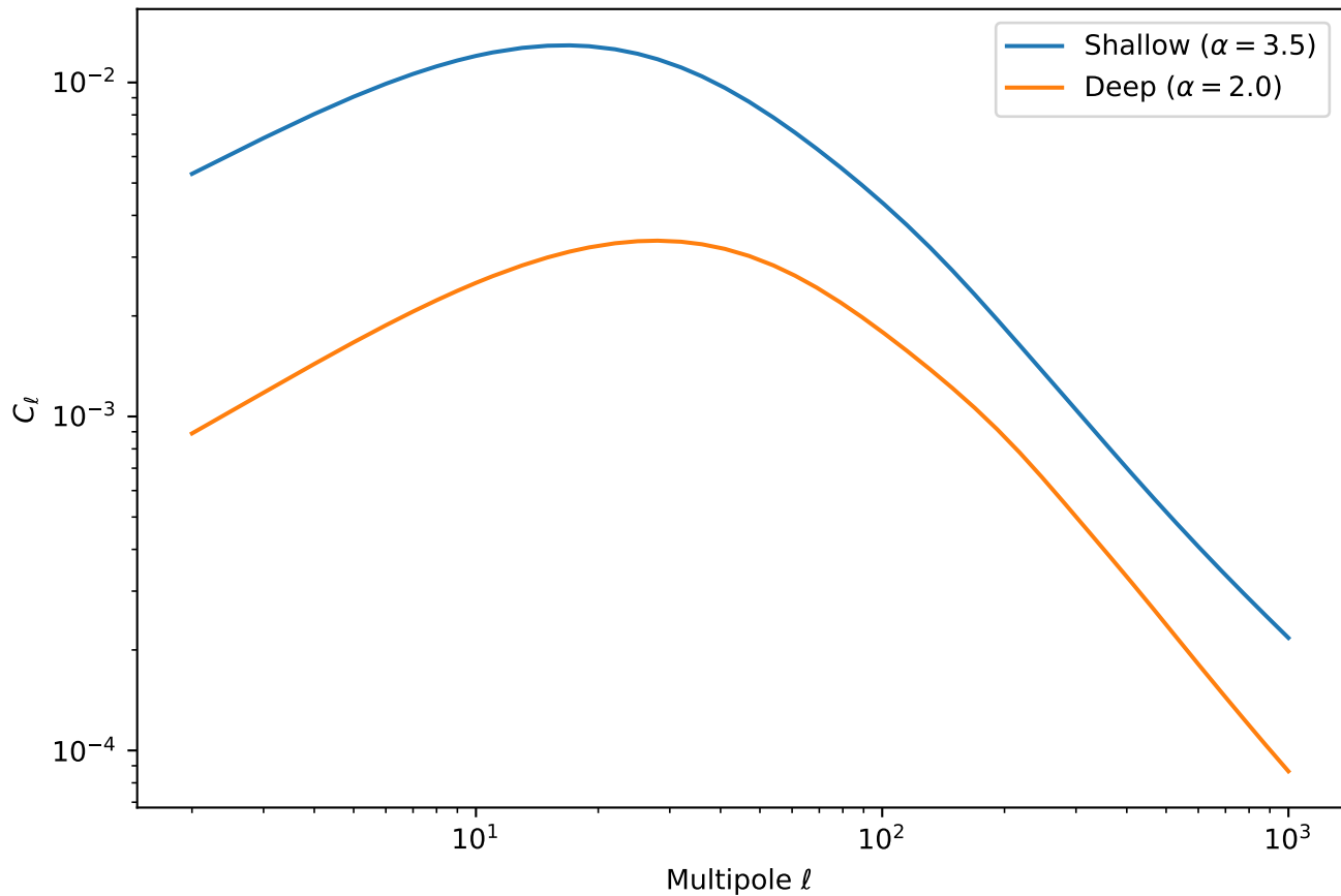
FRB Auto-Correlation: Shallow vs Deep Survey
