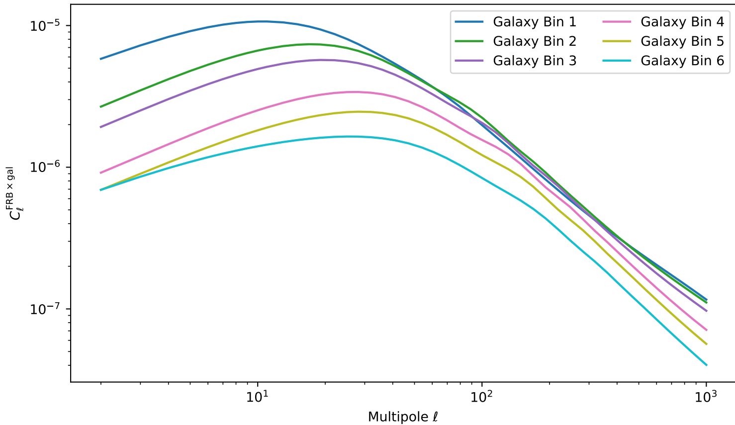
FRB×Galaxy — All Bins (Neutron Stars, Shallow Survey)
