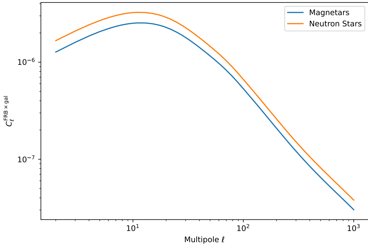
FRB Population Comparison (Deep Survey, Galaxy Bin 1)
