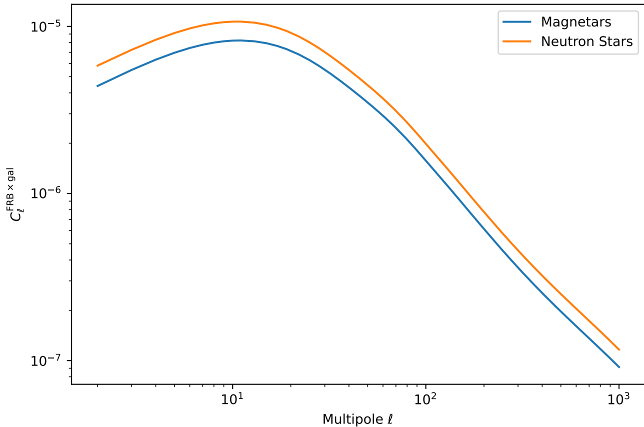
FRB Population Comparison (Shallow Survey, Galaxy Bin 1)
