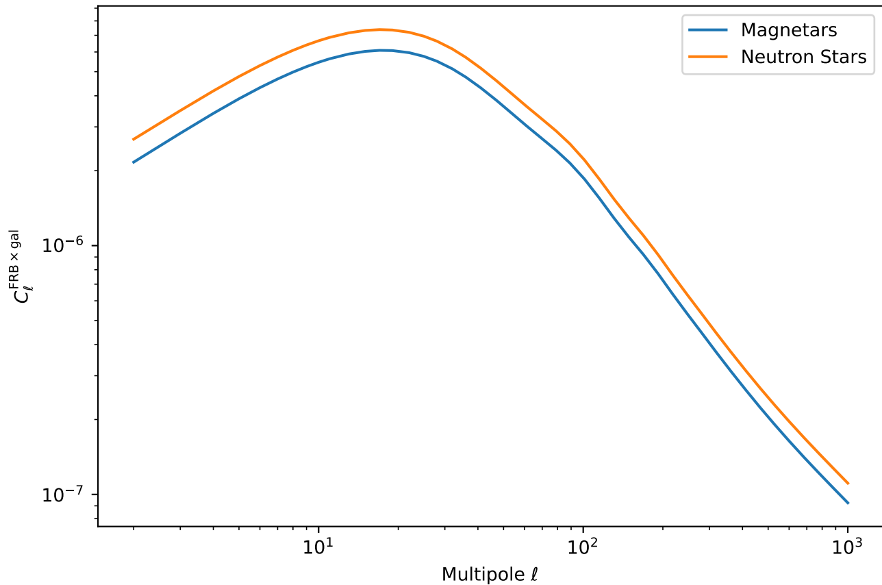
FRB Population Comparison (Shallow Survey, Galaxy Bin 2)
