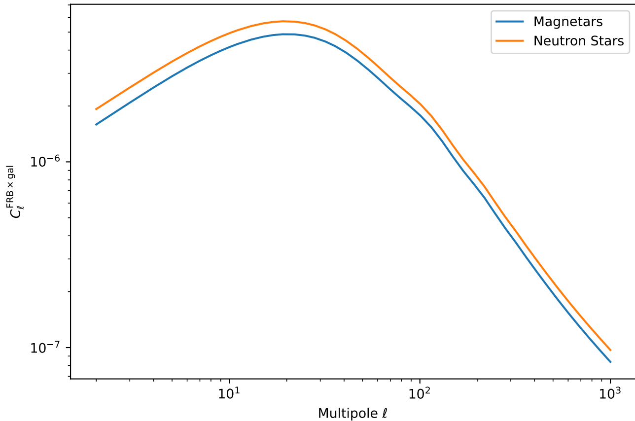
FRB Population Comparison (Shallow Survey, Galaxy Bin 3)
