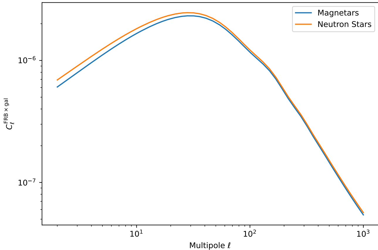
FRB Population Comparison (Shallow Survey, Galaxy Bin 5)
