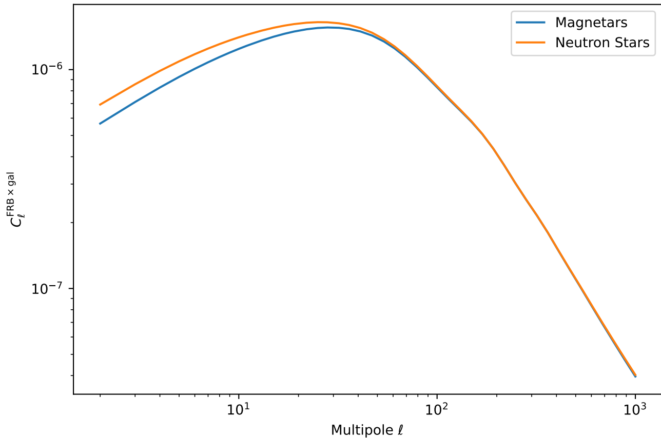
FRB Population Comparison (Shallow Survey, Galaxy Bin 6)
