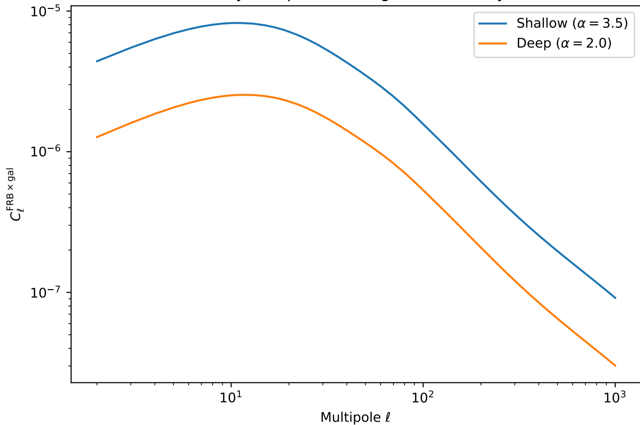
FRB Survey Comparison (Magnetars, Galaxy Bin 1)
