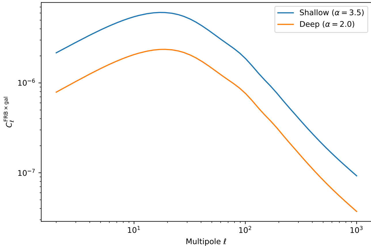
FRB Survey Comparison (Magnetars, Galaxy Bin 2)
