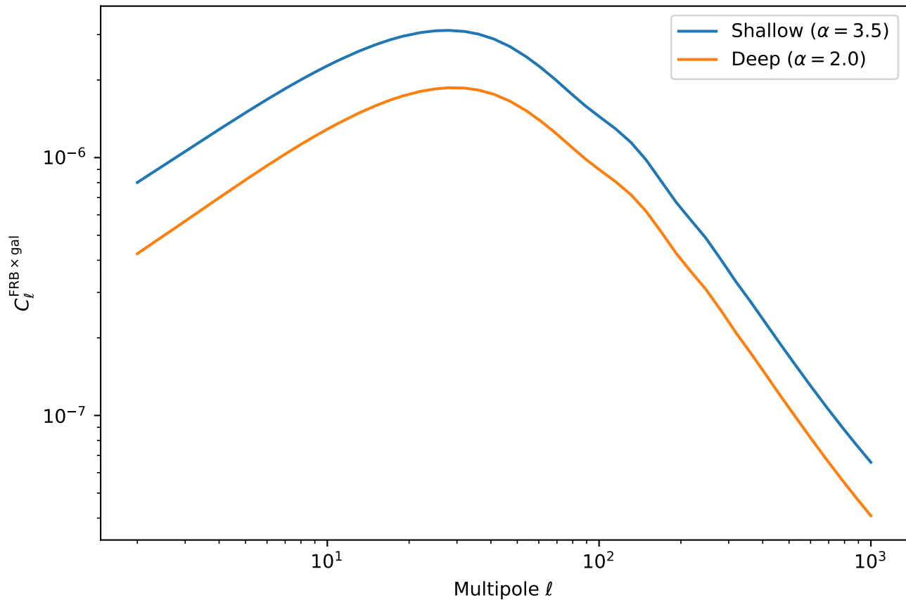
FRB Survey Comparison (Magnetars, Galaxy Bin 4)
