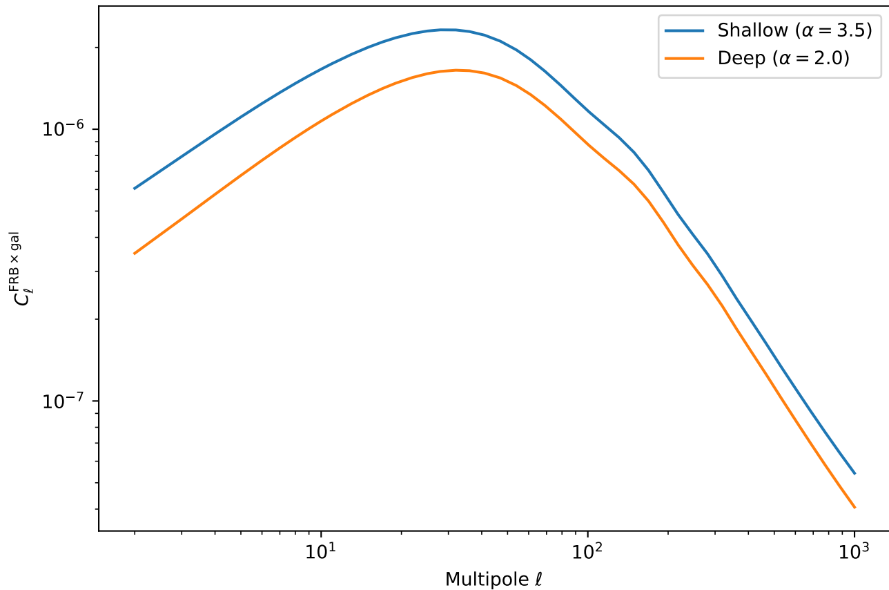
FRB Survey Comparison (Magnetars, Galaxy Bin 5)
