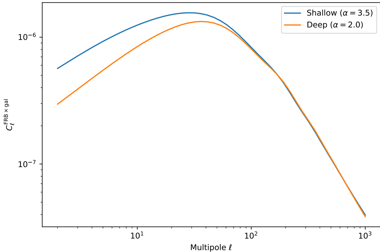
FRB Survey Comparison (Magnetars, Galaxy Bin 6)
