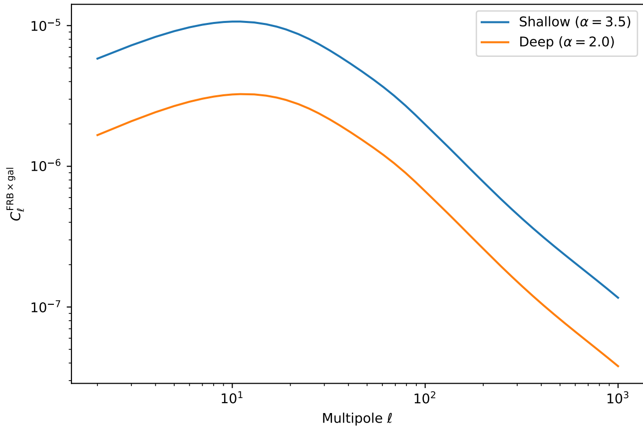
FRB Survey Comparison (Neutron Stars, Galaxy Bin 1)
