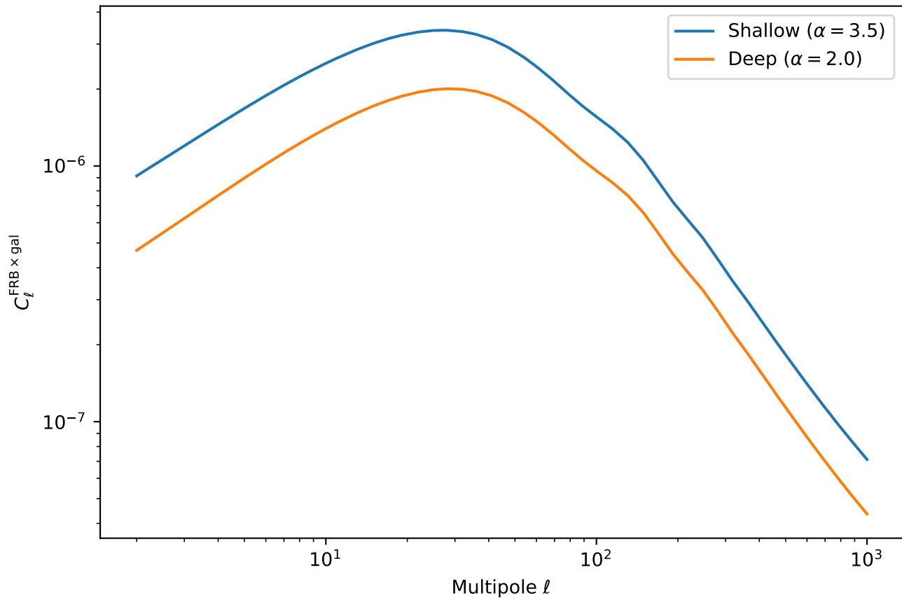
FRB Survey Comparison (Neutron Stars, Galaxy Bin 4)
