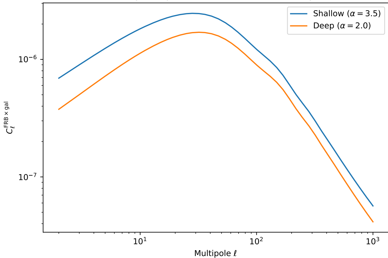
FRB Survey Comparison (Neutron Stars, Galaxy Bin 5)
