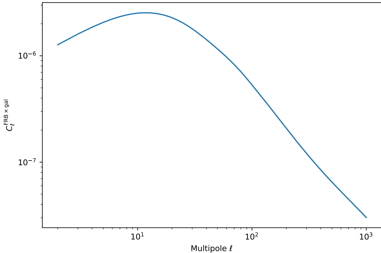
FRB×Galaxy Cross-Correlation (Magnetars, Deep Survey, Galaxy Bin 1)
