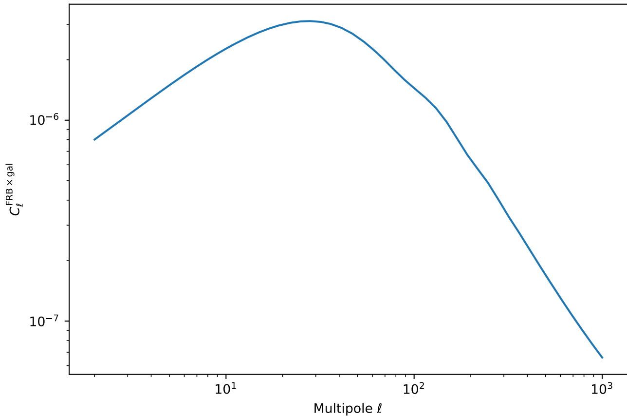
FRB×Galaxy Cross-Correlation (Magnetars, Shallow Survey, Galaxy Bin 4)
