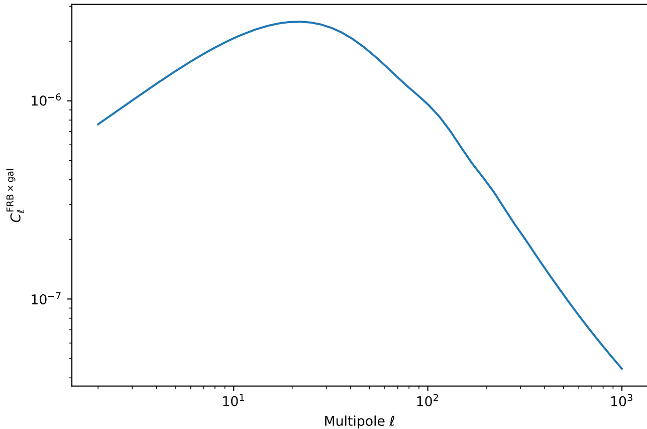
FRB×Galaxy Cross-Correlation (Neutron Stars, Deep Survey, Galaxy Bin 3)
