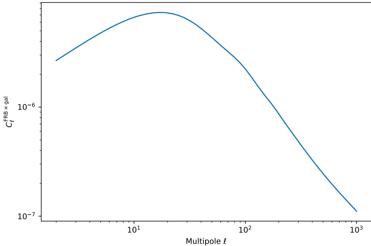
FRB×Galaxy Cross-Correlation (Neutron Stars, Shallow Survey, Galaxy Bin 2)
