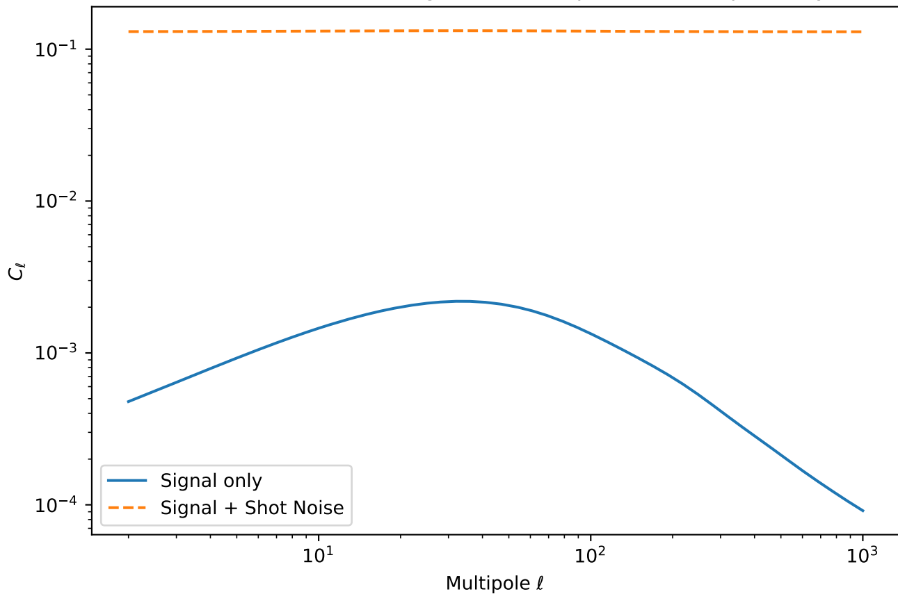
FRB Auto-Correlation Angular Power Spectrum (Deep Survey)
