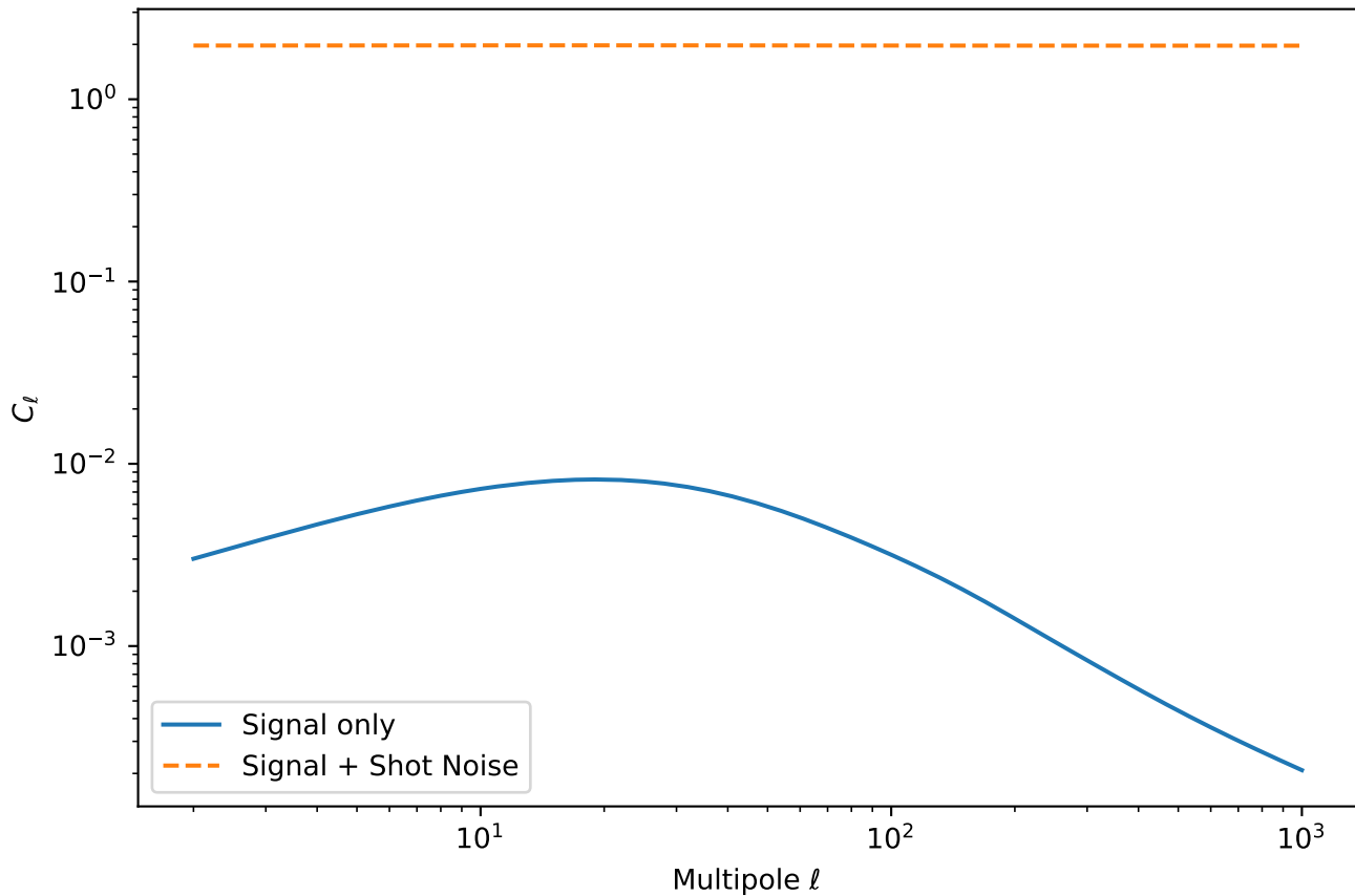
FRB Auto-Correlation Angular Power Spectrum (Shallow Survey)
