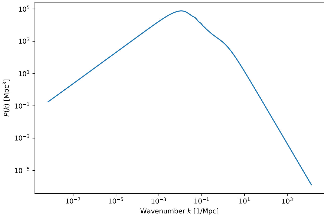
Nonlinear Matter Power Spectrum ( z = 0 )
