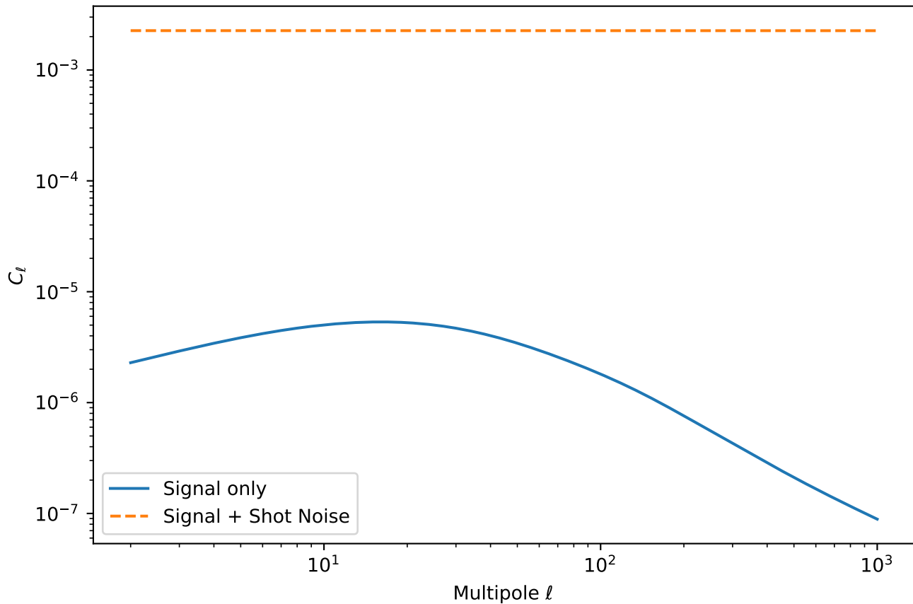
FRB Auto-Correlation Angular Power Spectrum (Shallow Survey) for Neutron Stars
