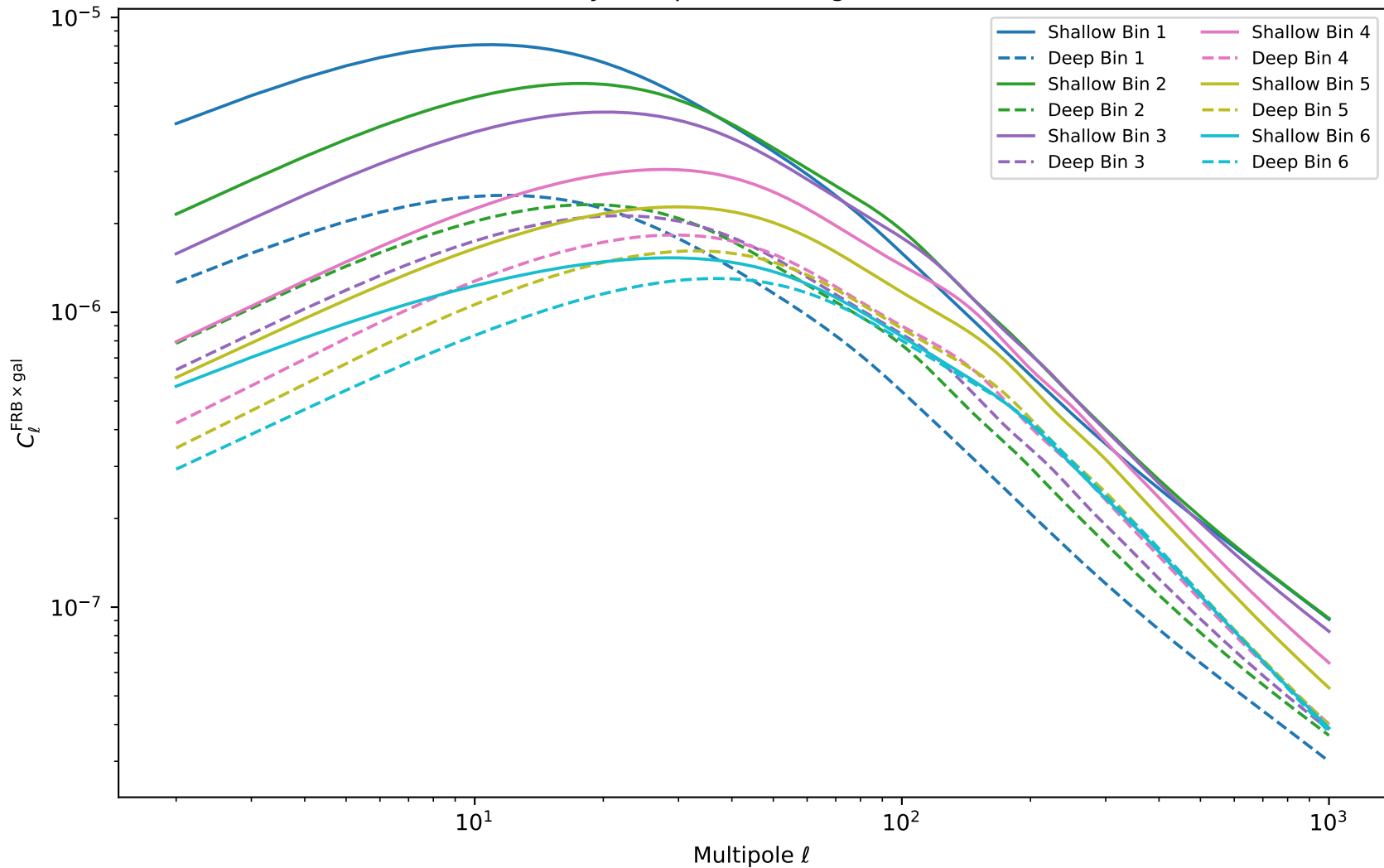
FRB Survey Comparison (Magnetars, all bins)
