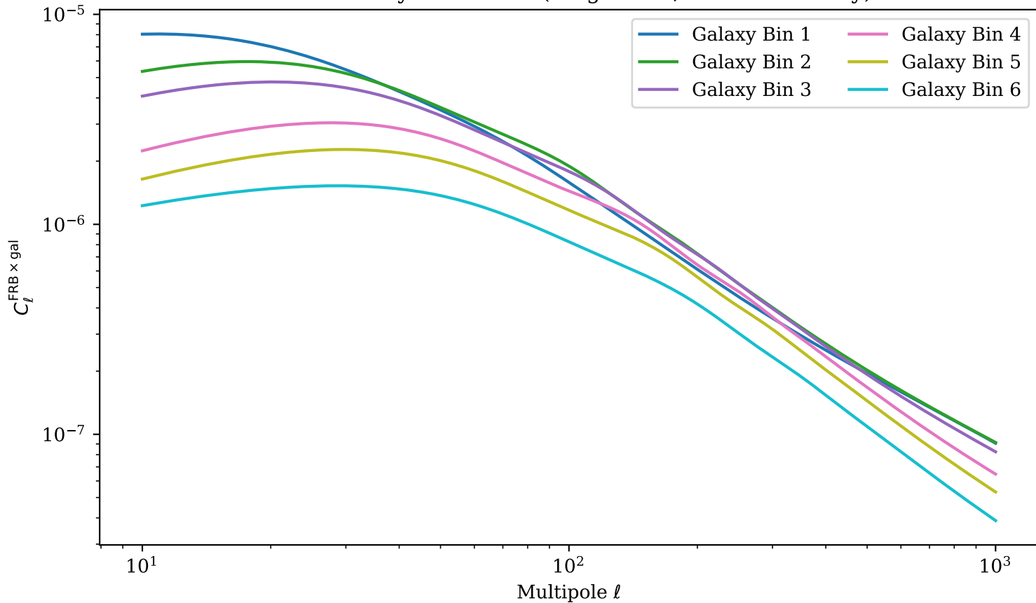
FRB×Galaxy — All Bins (Magnetars, Shallow Survey)
