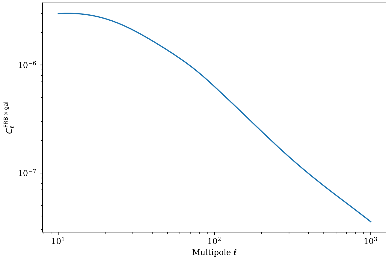
FRB×Galaxy Cross-Correlation (Neutron Stars, Deep Survey, Galaxy Bin 1)
