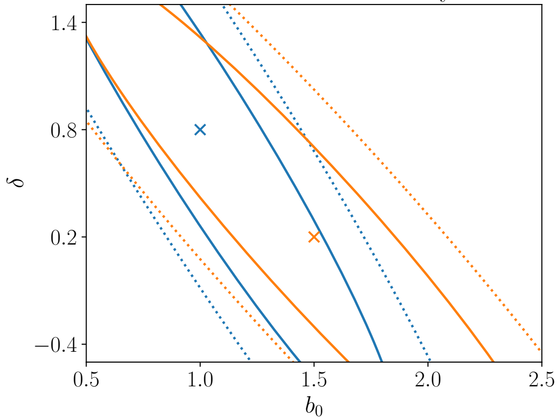
LSST Y10 Shallow Survey
