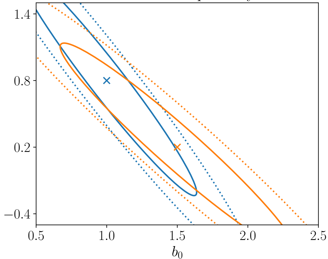
LSST Y10 Deep Survey
