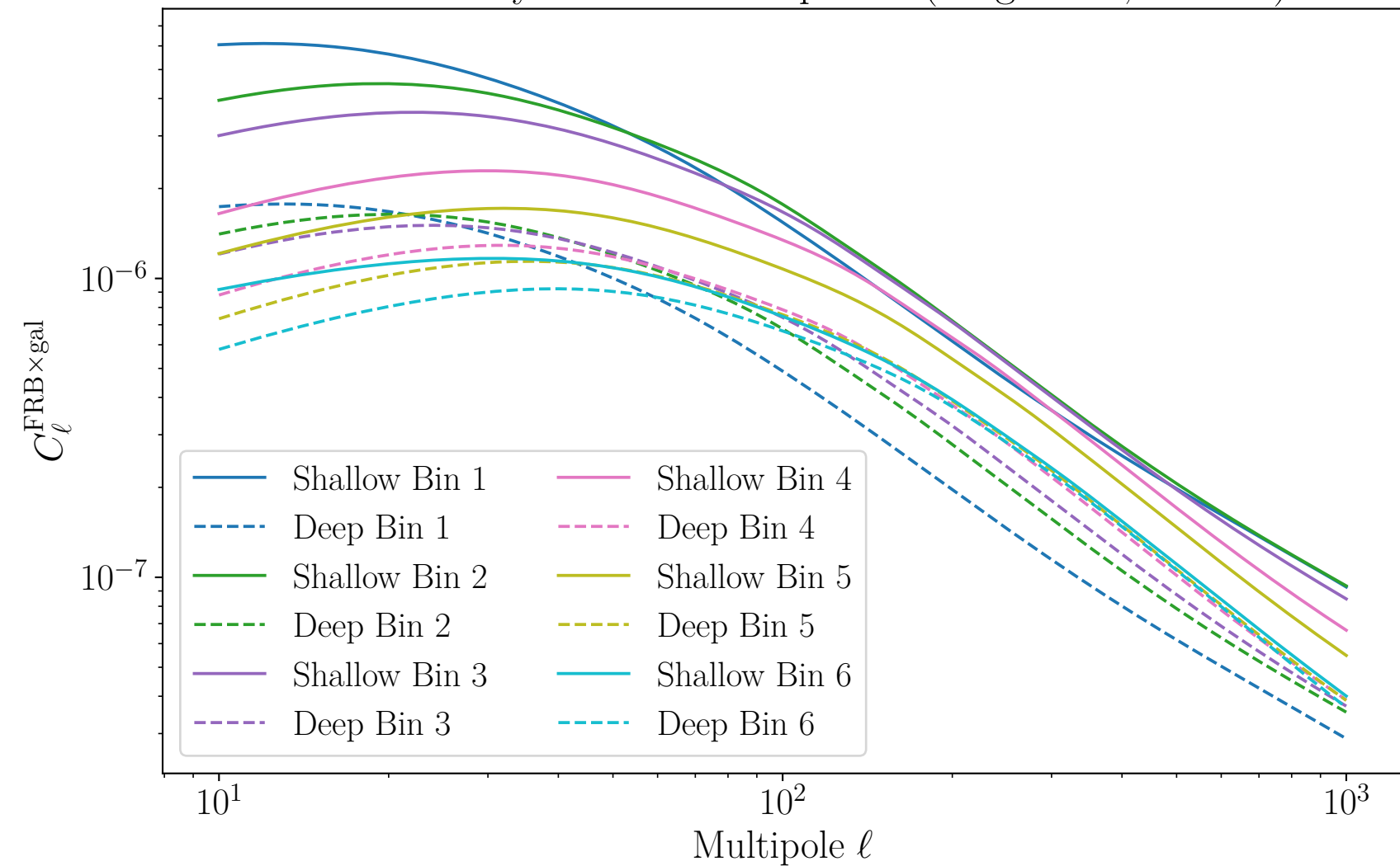
FRB x Galaxy Cross-Power Spectra (Magnetars, all bins)
