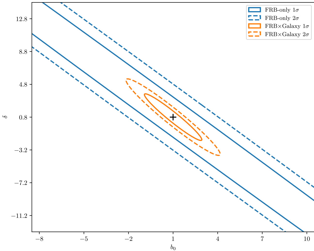
Fisher Forecast — Magnetars, Deep Survey Fiducial: b_0 = 1.0 , \delta = 0.8
