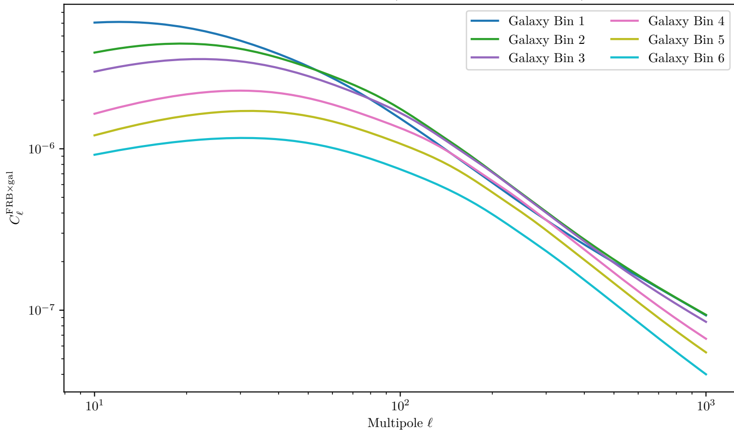
FRB×Galaxy — All Bins (Magnetars, Shallow Survey)
