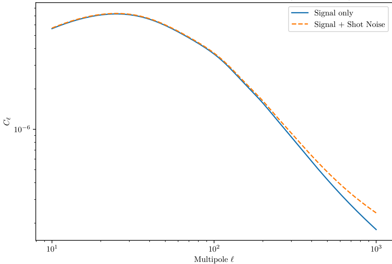
Galaxy Auto-Correlation Angular Power Spectrum (Bin 3 x Bin 3)
