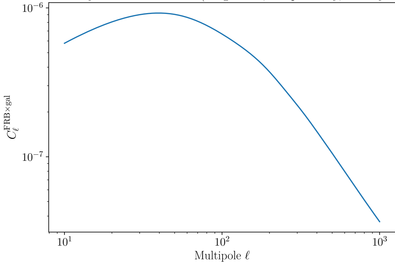
FRB \times Galaxy Cross-Correlation (Magnetars, Deep Survey, Galaxy Bin
