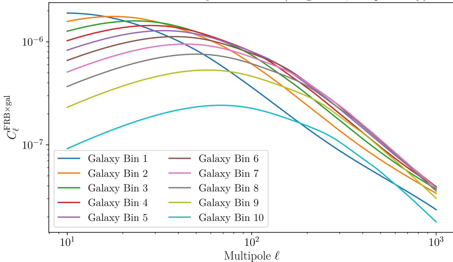
LSST Y10 FRB×Galaxy — All Bins (Magnetars, Deep Survey)
