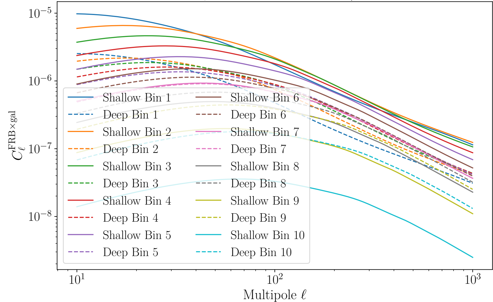
LSST Y10 FRB x Galaxy Cross-Power Spectra (Neutron Stars, all bins)
