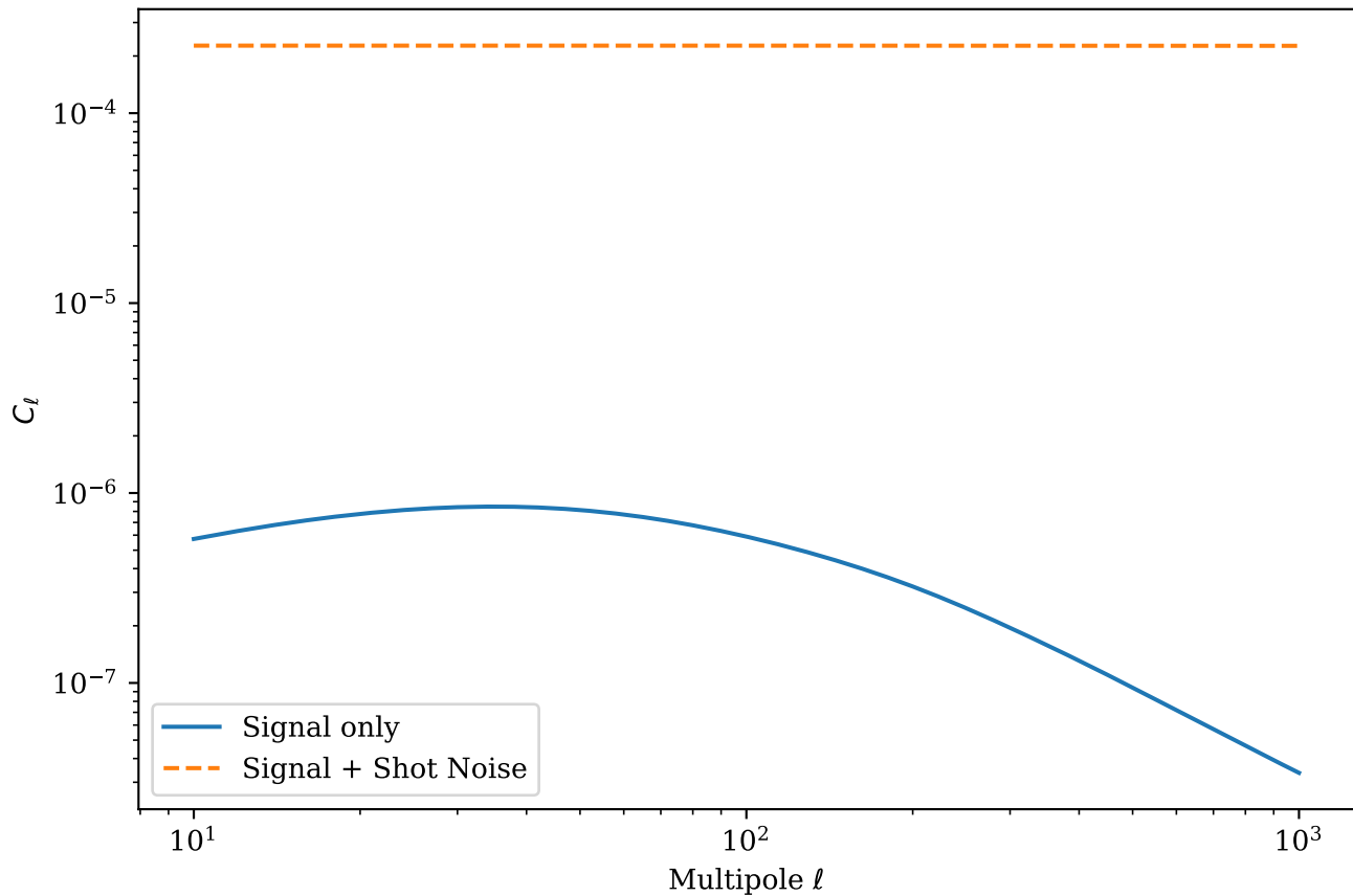
FRB Auto-Correlation Angular Power Spectrum (Deep Survey) for Magnetar
