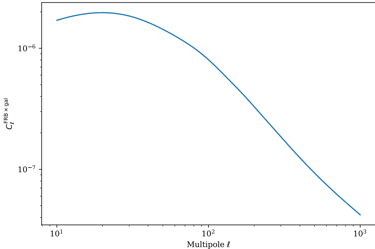
FRB×Galaxy Cross-Correlation (Neutron Stars, Deep Survey, Galaxy Bin 2)
