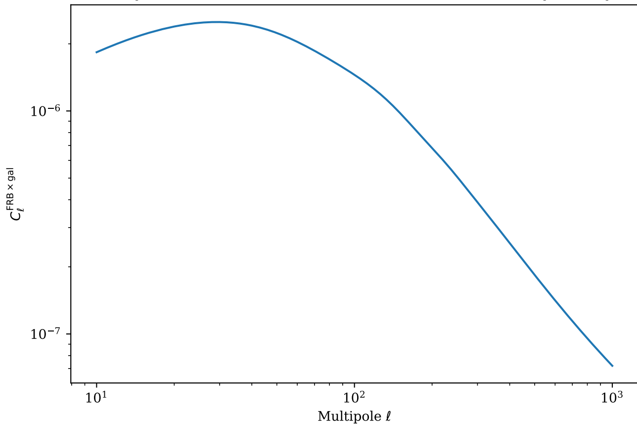
FRB×Galaxy Cross-Correlation (Neutron Stars, Shallow Survey, Galaxy Bin .
