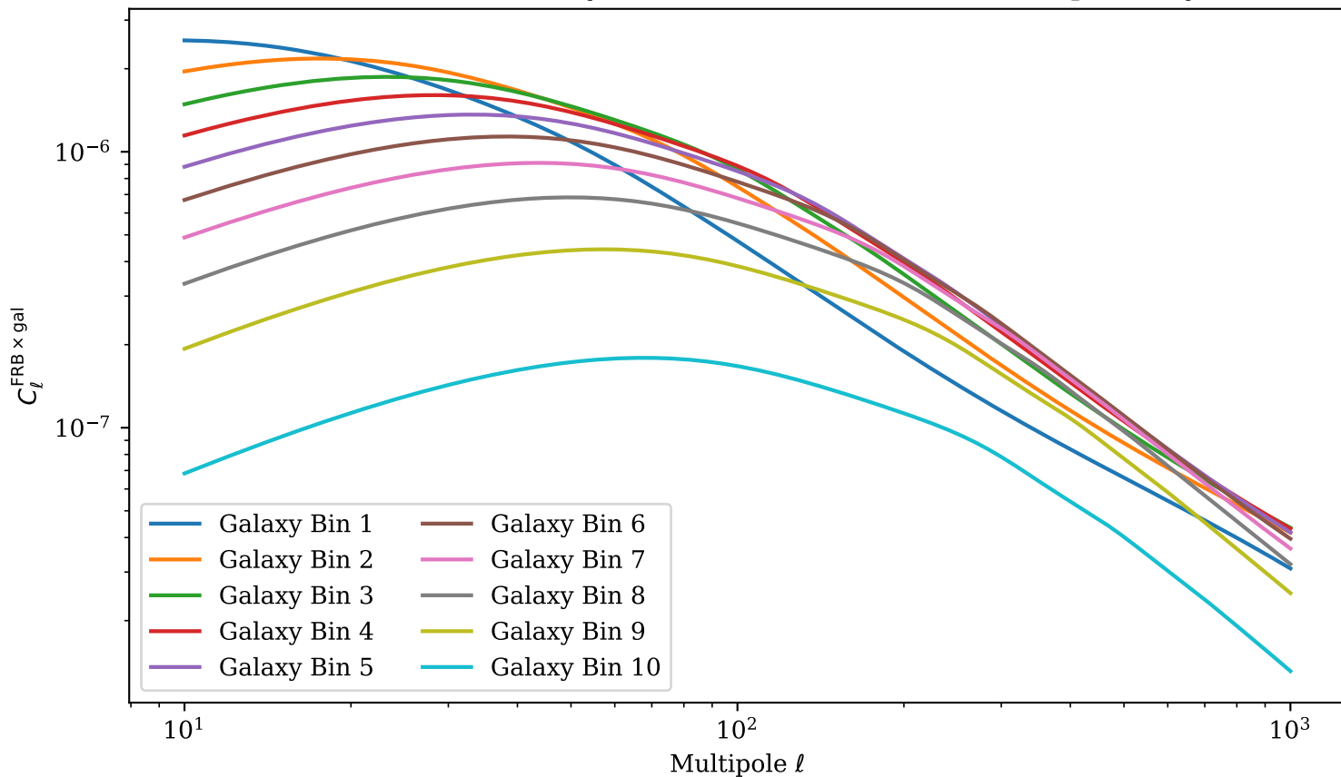
LSST Y10 FRB×Galaxy — All Bins (Neutron Stars, Deep Survey)
