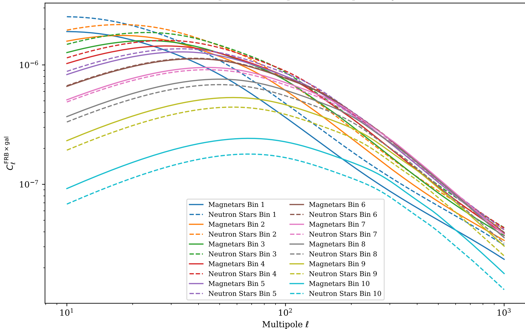
LSST Y10 FRB Population Comparison (Deep Survey, all bins)
