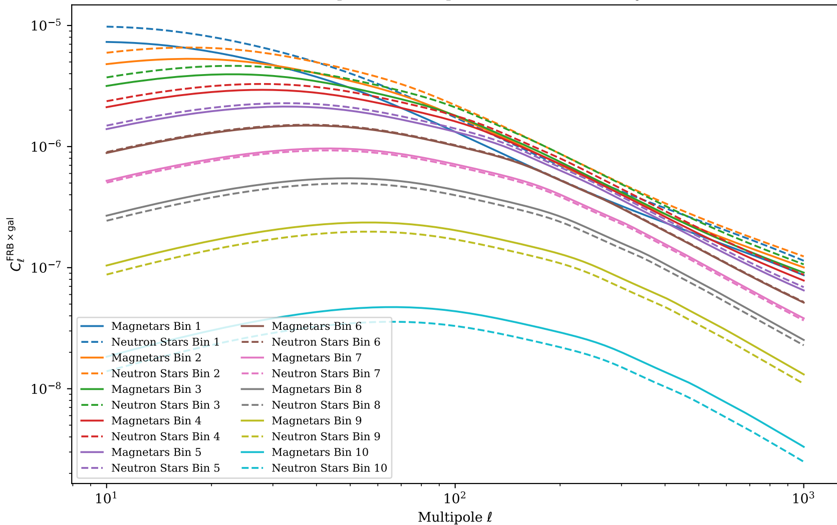
LSST Y10 FRB Population Comparison (Shallow Survey, all bins)
