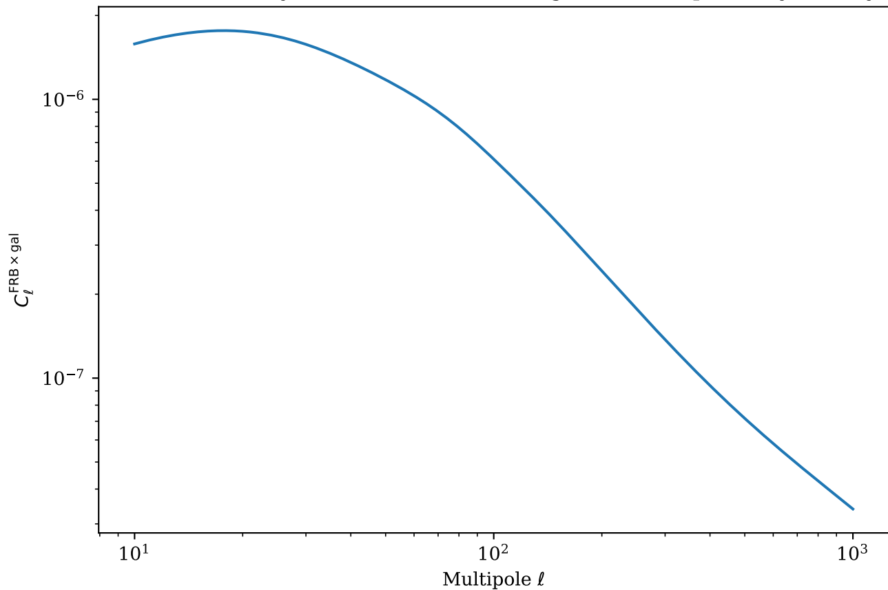
LSST Y10 FRB×Galaxy Cross-Correlation (Magnetars, Deep Survey, Galaxy Bi
