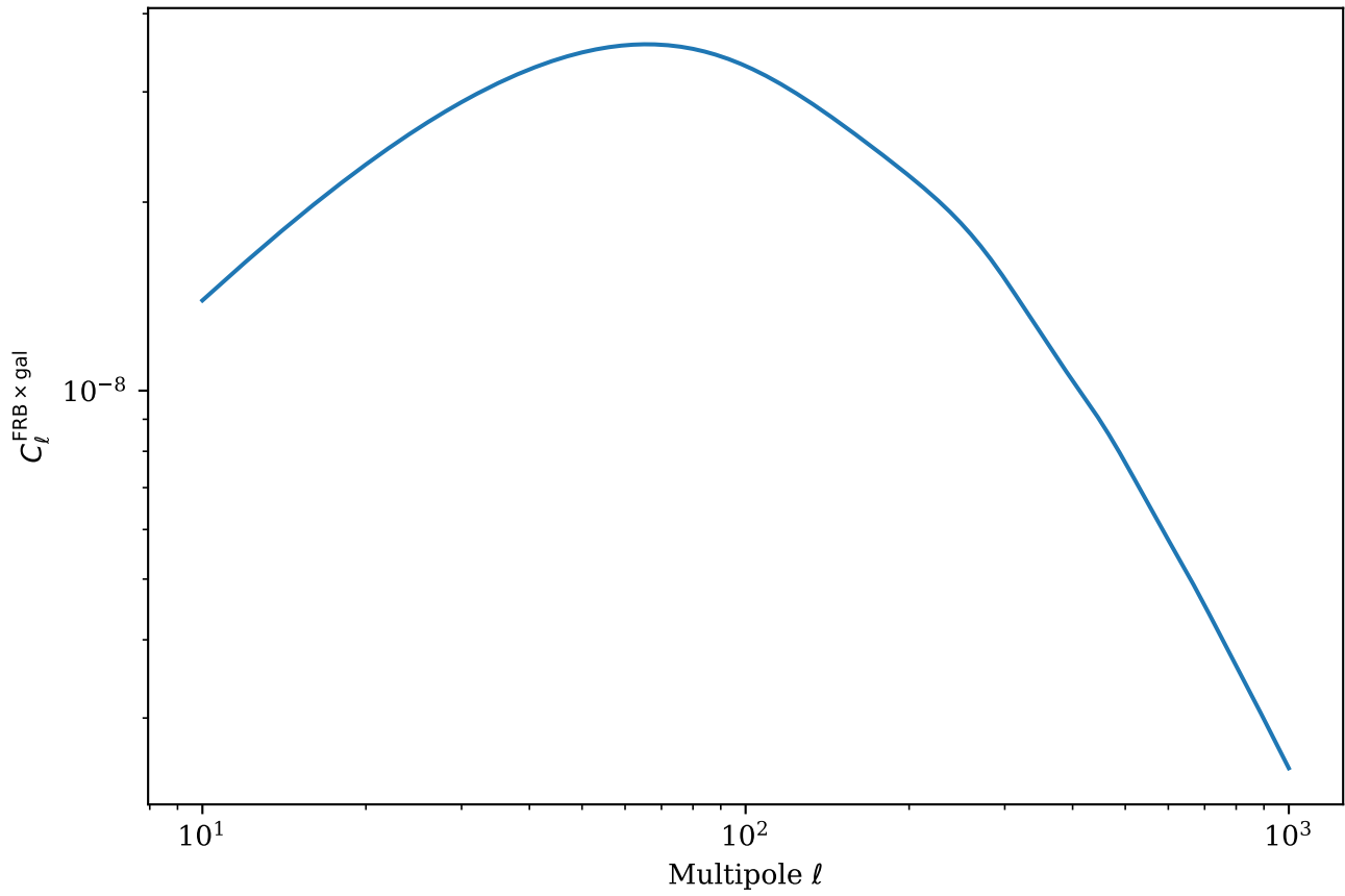
LSST Y10 FRB×Galaxy Cross-Correlation (Neutron Stars, Shallow Survey, Galaxy
