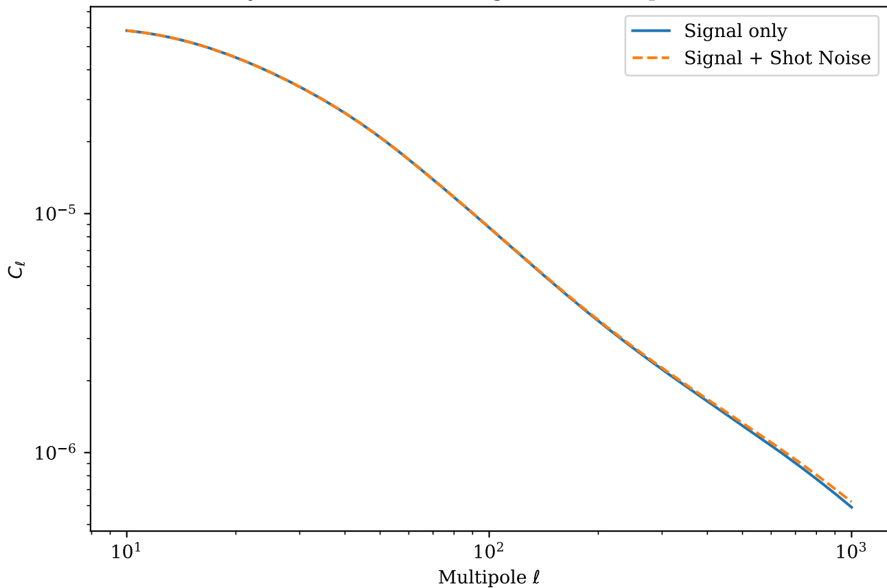
LSST Y10 Galaxy Auto-Correlation Angular Power Spectrum (Bin 1 x Bin 1)
