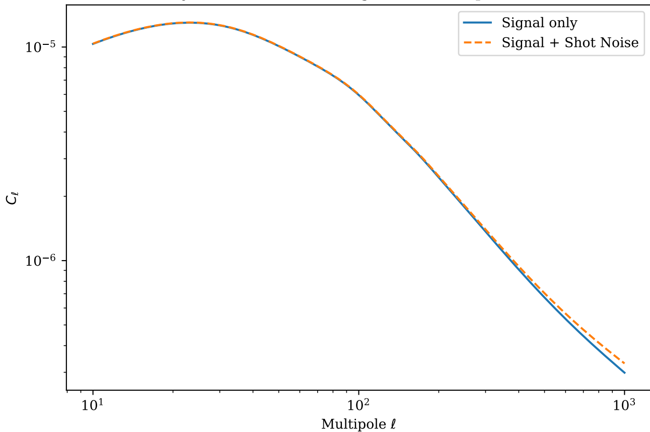
LSST Y10 Galaxy Auto-Correlation Angular Power Spectrum (Bin 3 x Bin 3)
