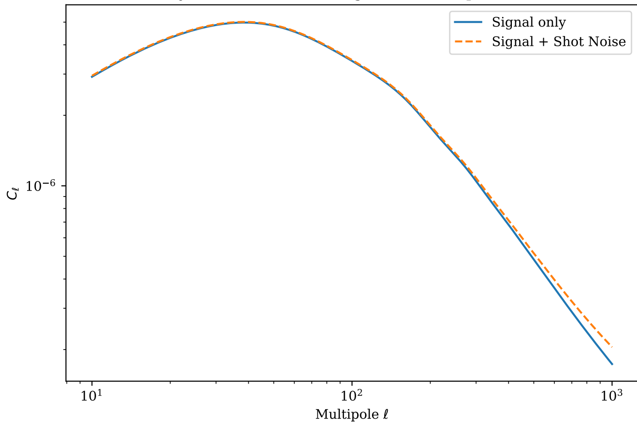
LSST Y10 Galaxy Auto-Correlation Angular Power Spectrum (Bin 6 x Bin 6)
